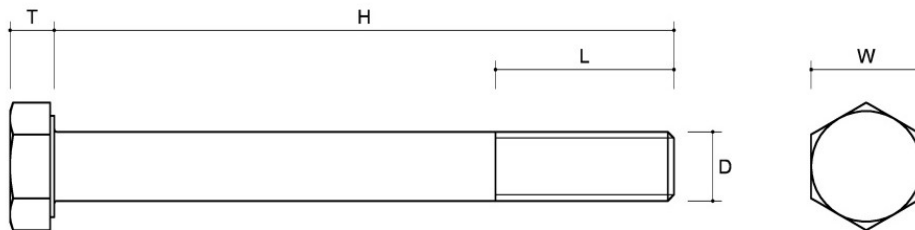
Figure 68 Bolt type M12x35
