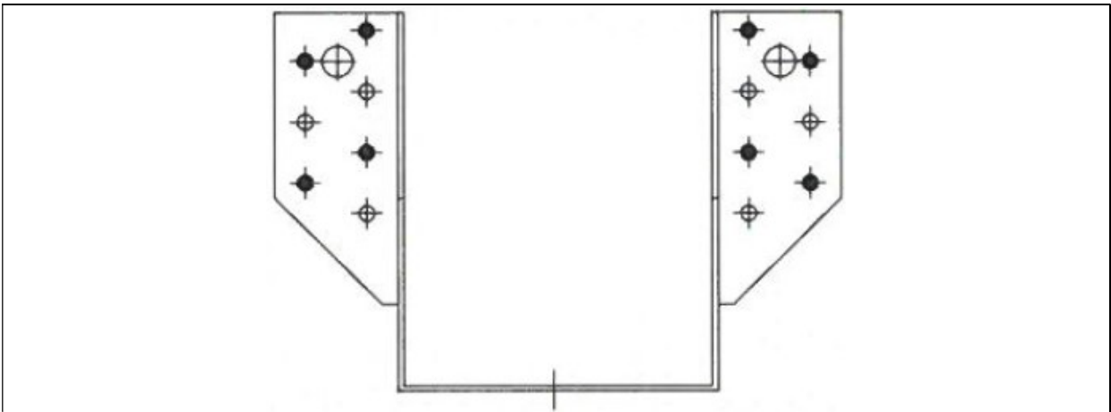
Figure 159 Type WB 1, WB 2, WB 5, WB 8, WB 10, WB 14, WB 19
